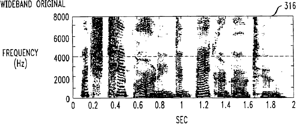
FIG. 17D WIDEBAND ORIGINAL
