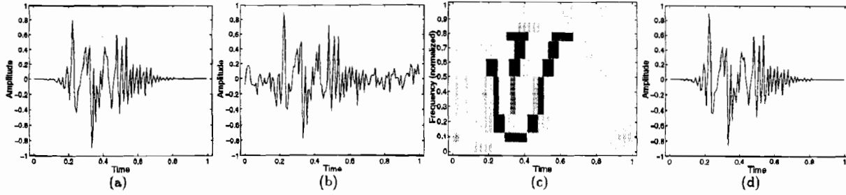
Figure 1. MDL-based translation-invariant denoising: (a) Synthetic signal; (b) Noisy measurement with SNR= 7dB; (c) SIWPD of the noisy measurement using the MDL criterion; (d) Signal estimate, SNR= 19dB.
